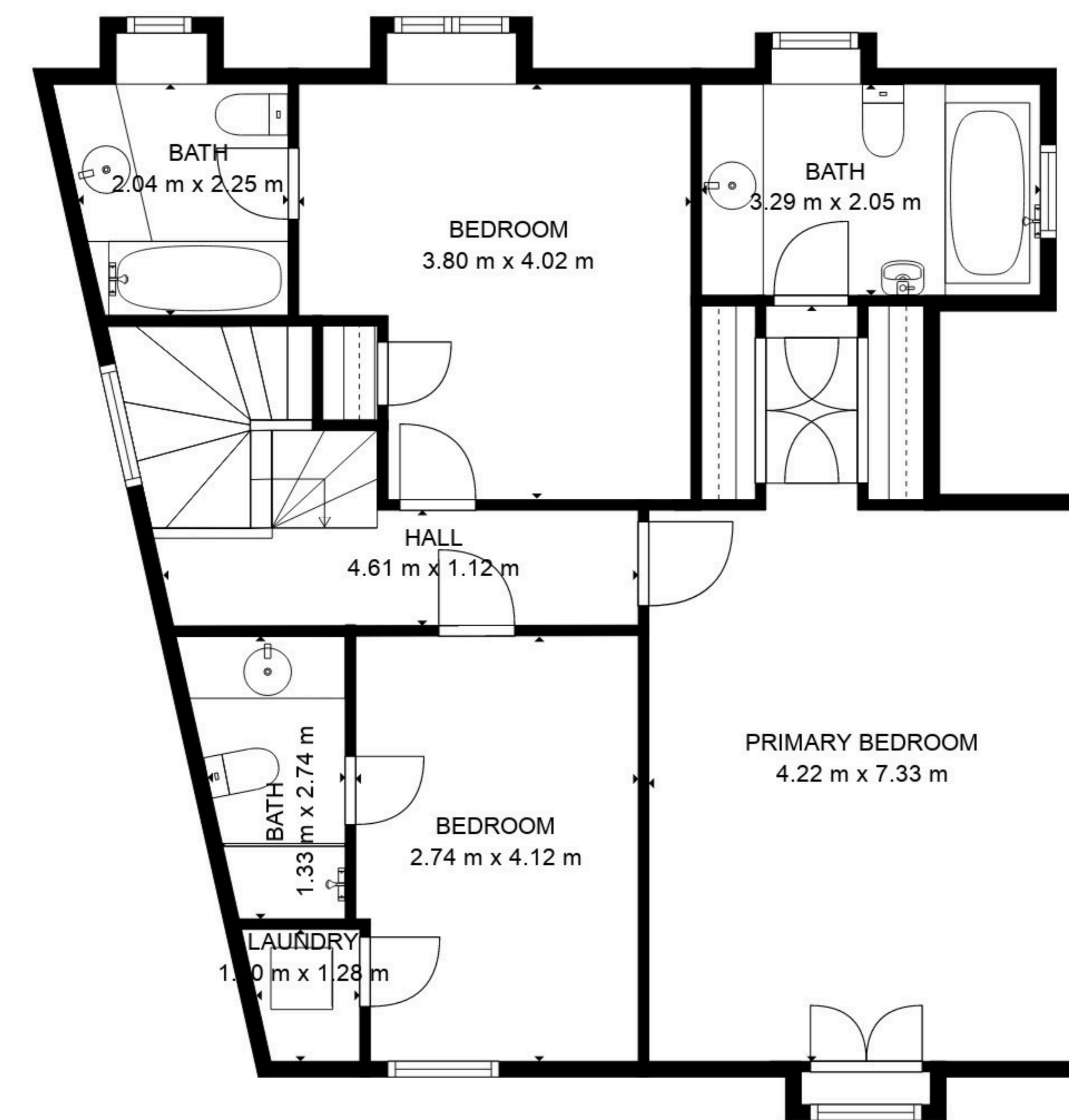
FLOOR 2
